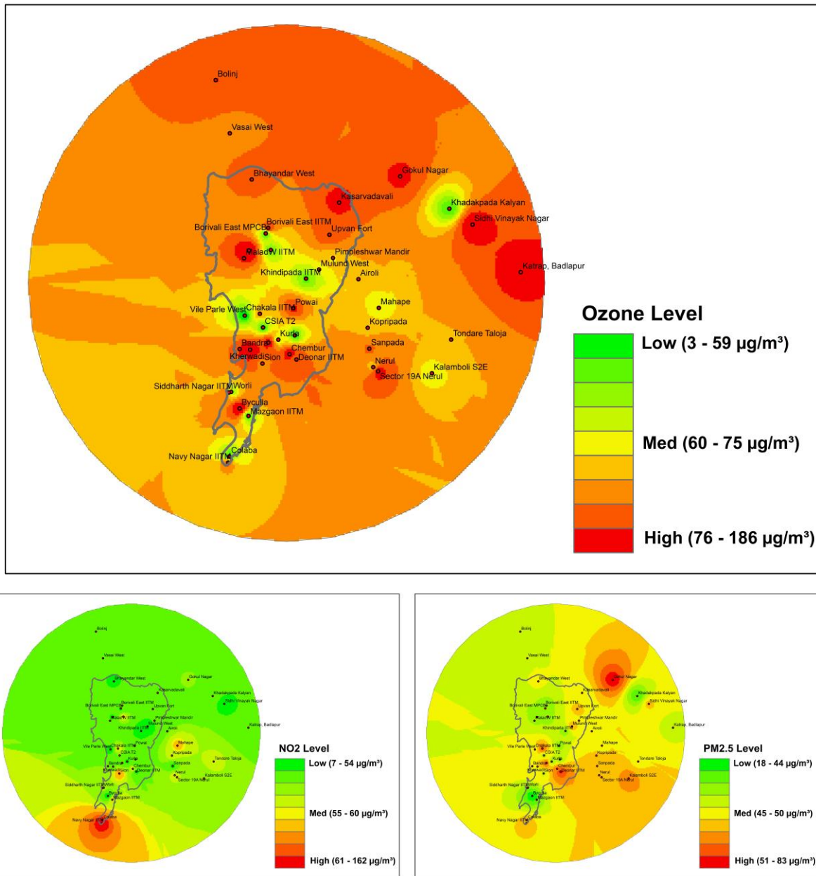
Map 2: Spatial relationship among hotspots for key pollutants in MMR
