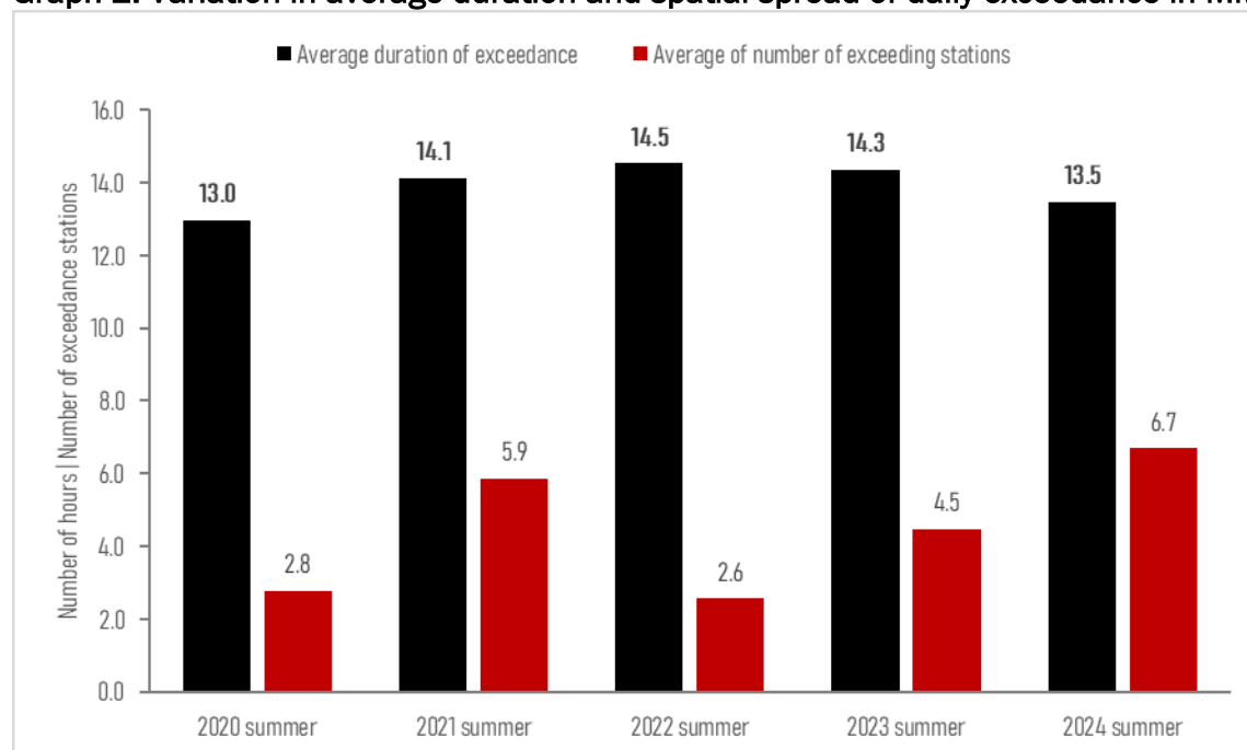
Graph 2: Variation in average duration and spatial spread of daily exceedance in MMR
