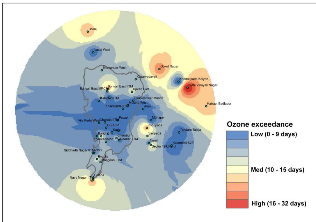
Map 1: Hotspots of ground-level ozone exceedance in Mumbai Metropolitan Region
