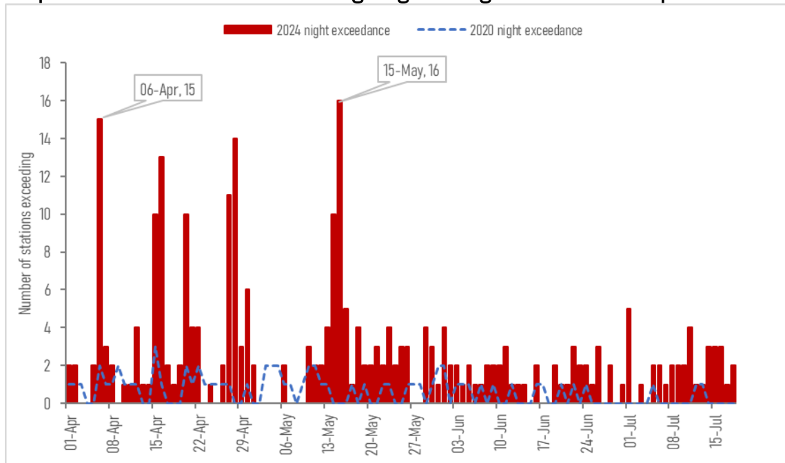
Graph 4: Variation in occurrence of high night-time ground-level ozone pollution
