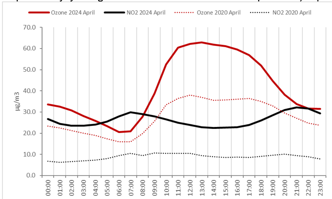
Graph 3: Hourly cycle of ground-level ozone and NO 2 in MMR – April 2020 v/s April 2024
