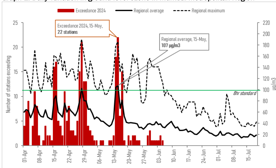
Graph 1: Daily variation in ground-level ozone in Mumbai Metropolitan Region
