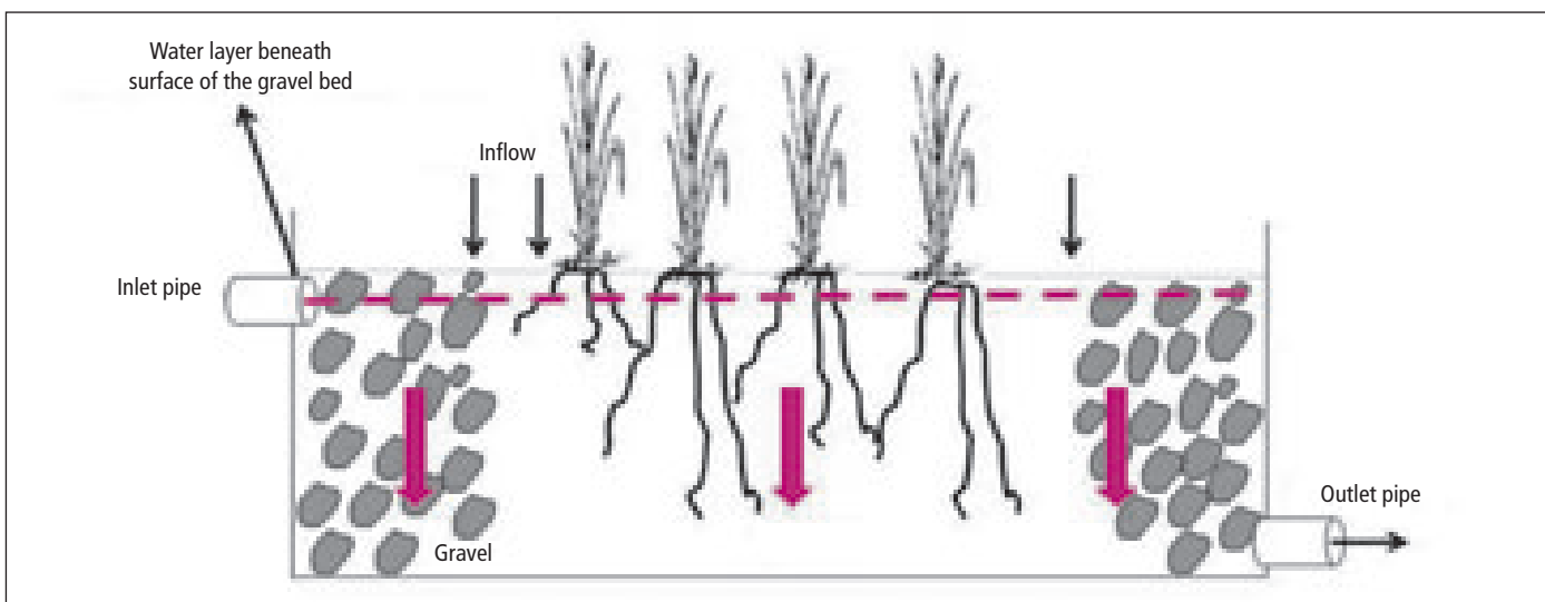
DIAGRAM 4 Cross-sectional view of the horizontal sub-surface flow
