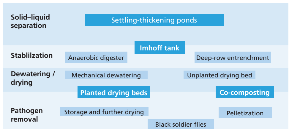
Figure 8: Different treatment technologies based on their function
